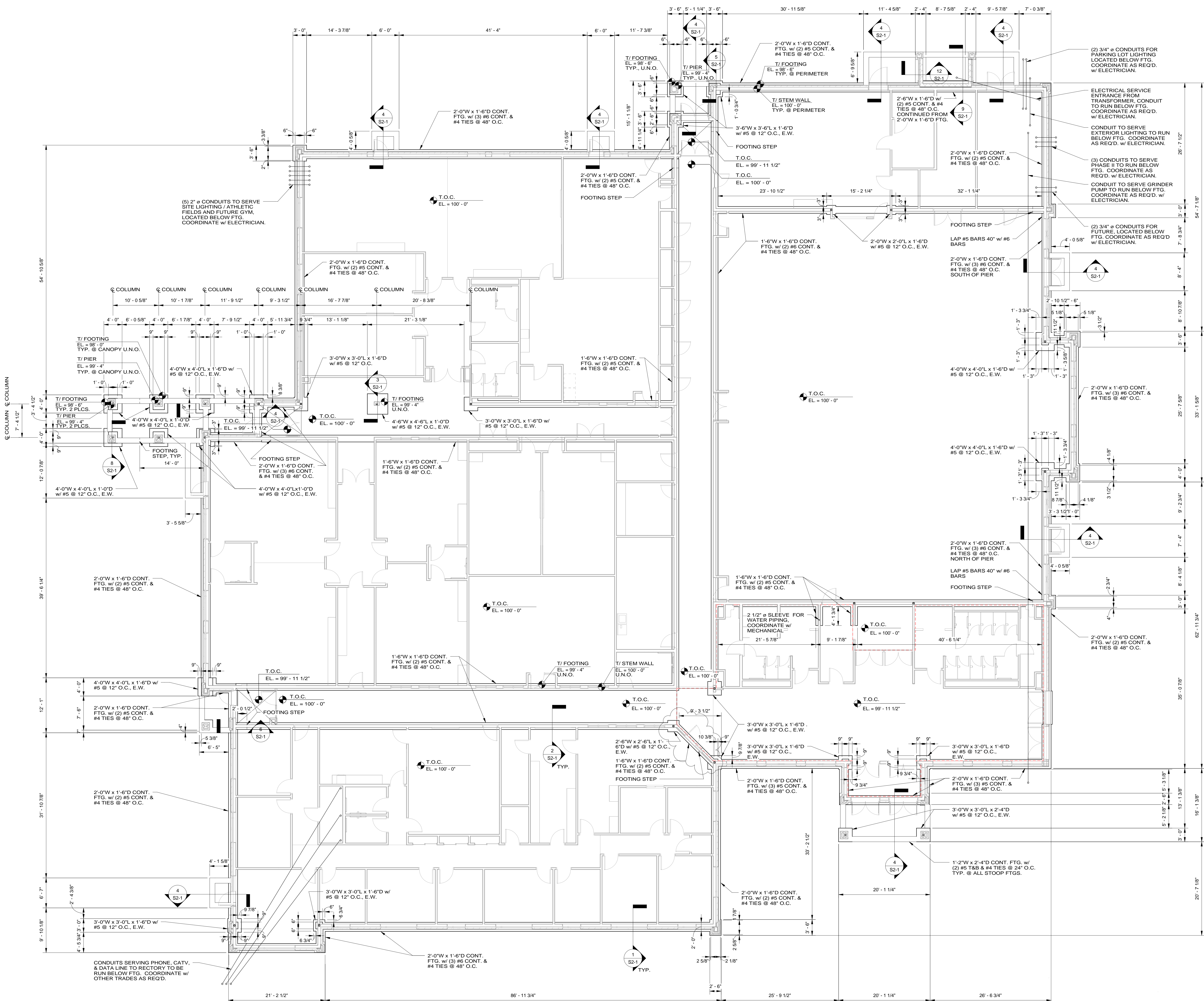
1 Footing Plan 1/8" = 1'-0"
