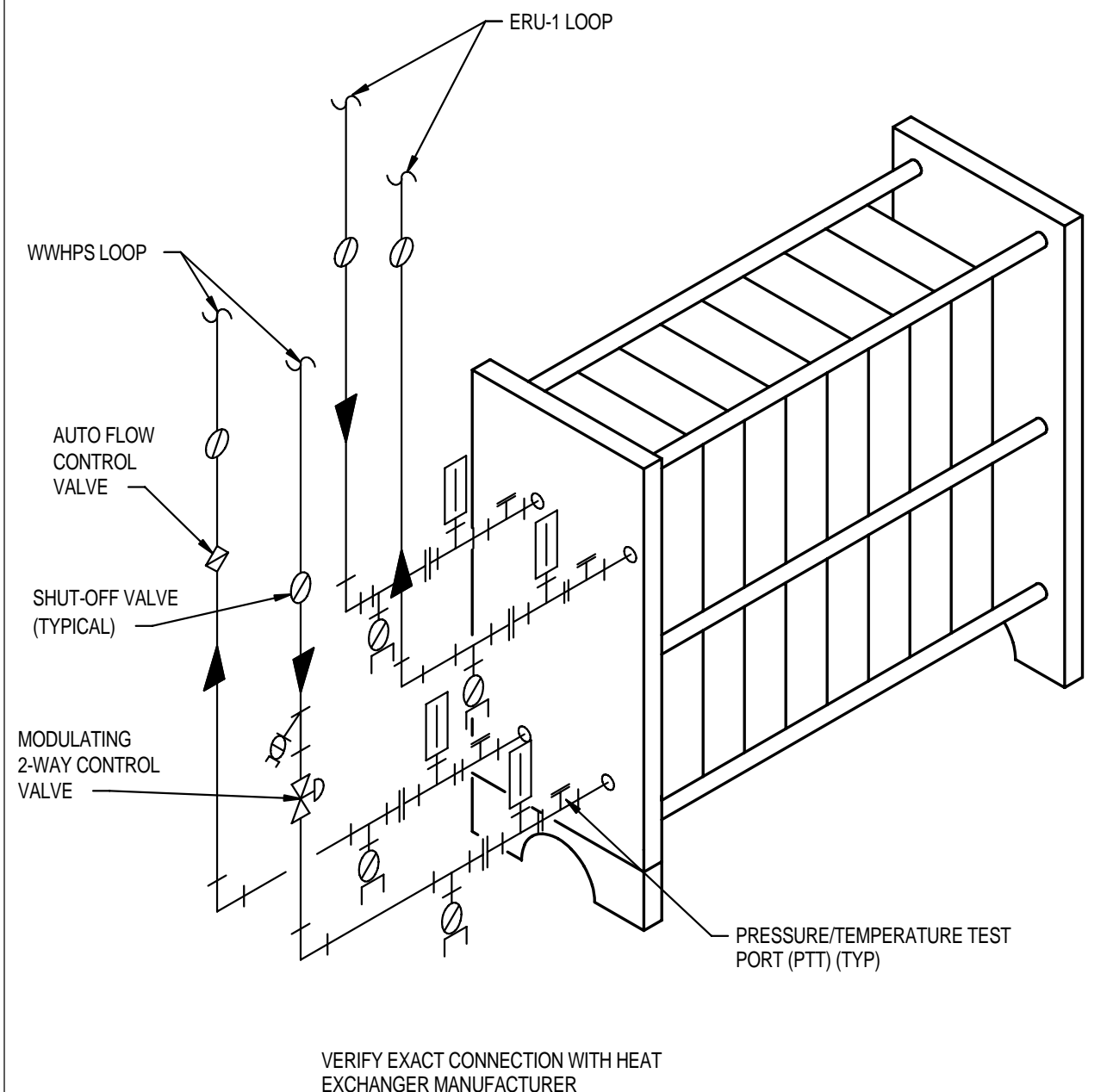
WATER TO WATER HEAT EXCHANGER DETAIL NO SCALE (10) M4-0
