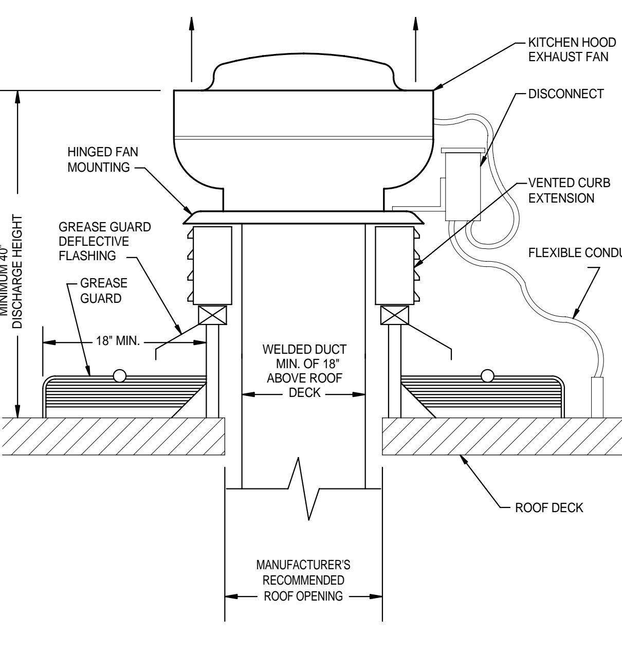
KITCHEN HOOD EXHAUST FAN DETAIL NO SCALE (3) M4-0
