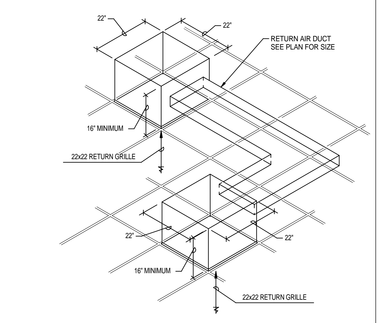
TRANSFER GRILLE CONNECTION DETAIL NO SCALE (7) M4-0
