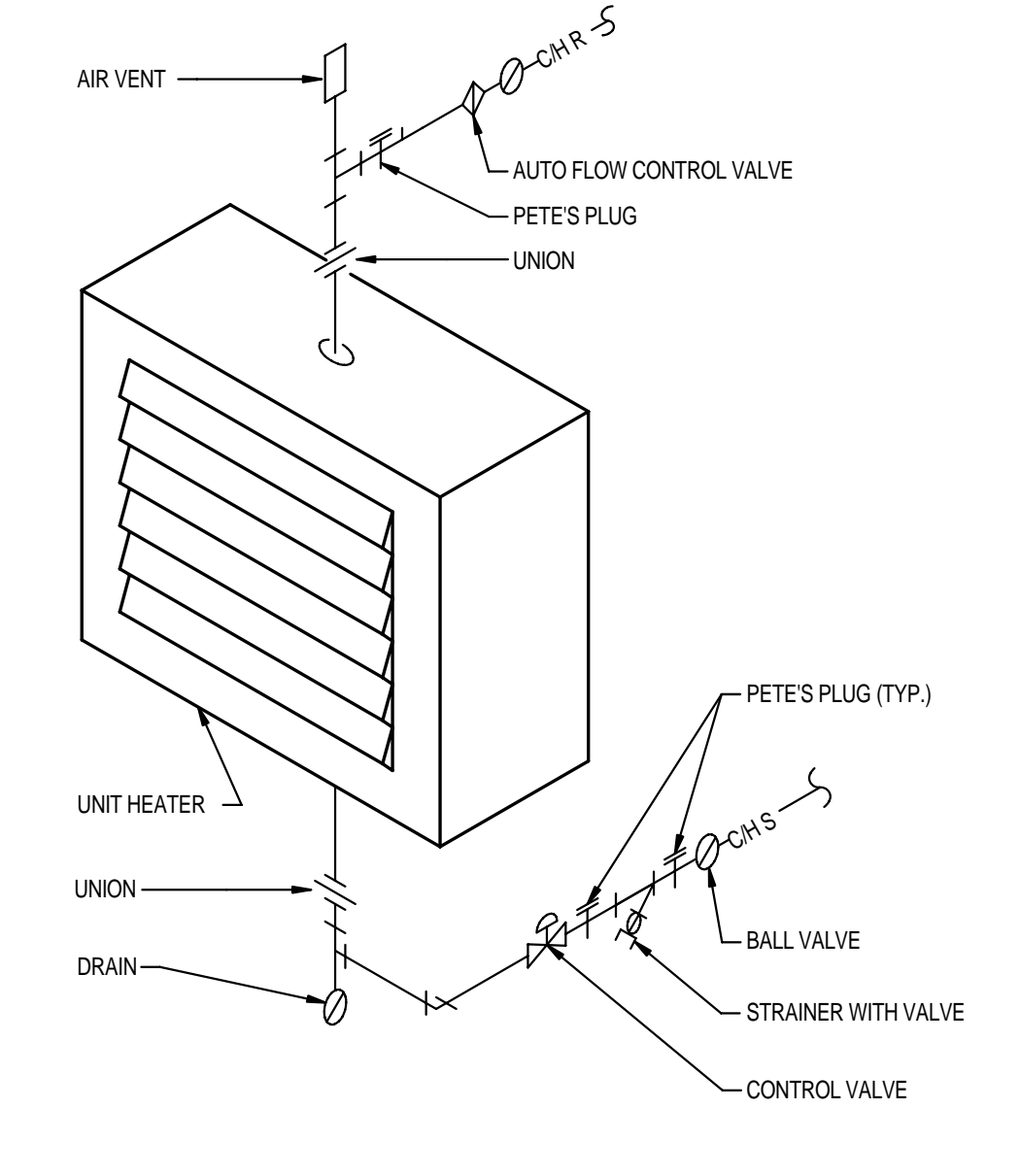
HOT WATER UNIT HEATER DETAIL NO SCALE (13) M4-0
