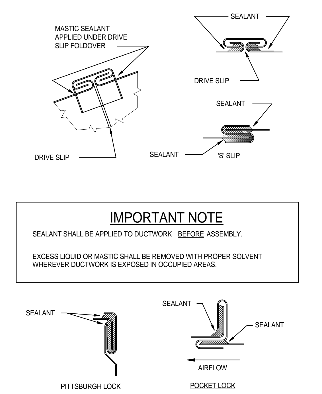
DUCTWORK SEALANT DETAIL NO SCALE (1) M4-0
