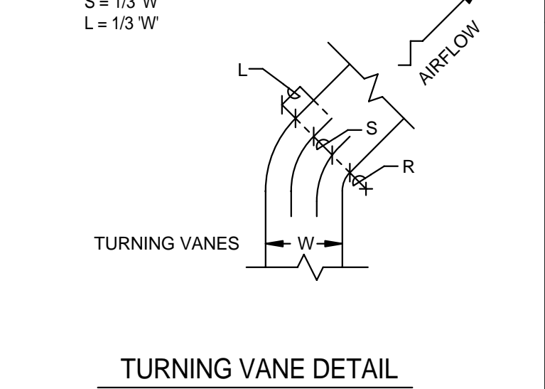
TURNING VANE DETAIL
