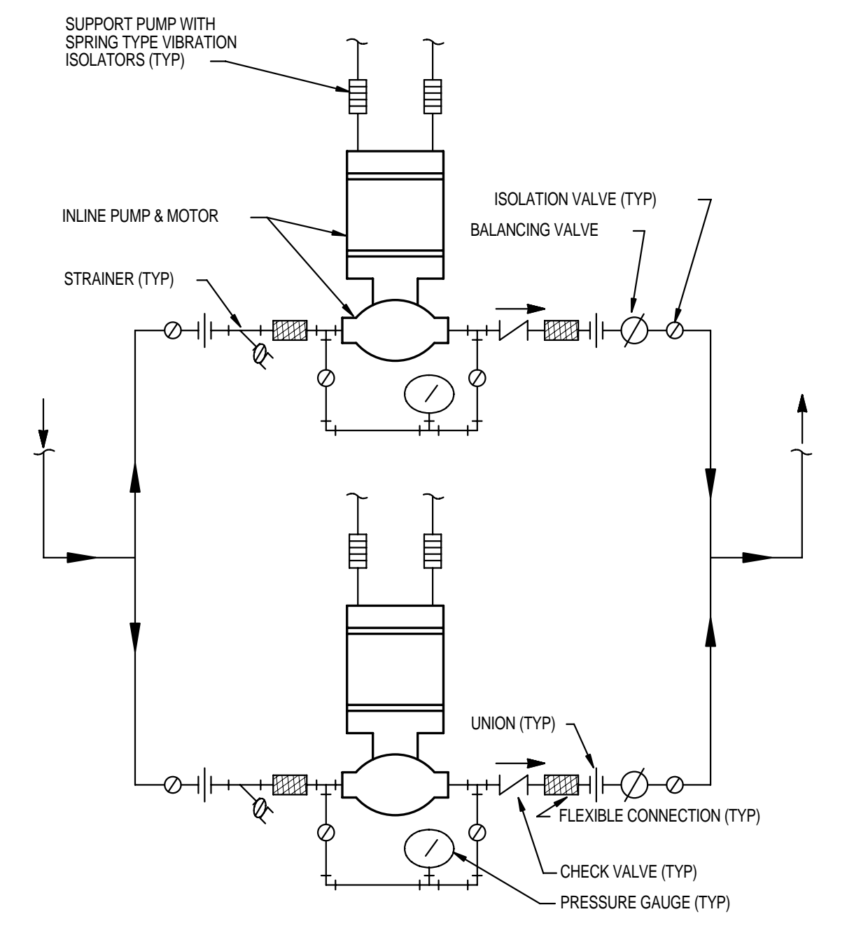
INLINE PUMP DETAIL NO SCALE (12) M4-0
