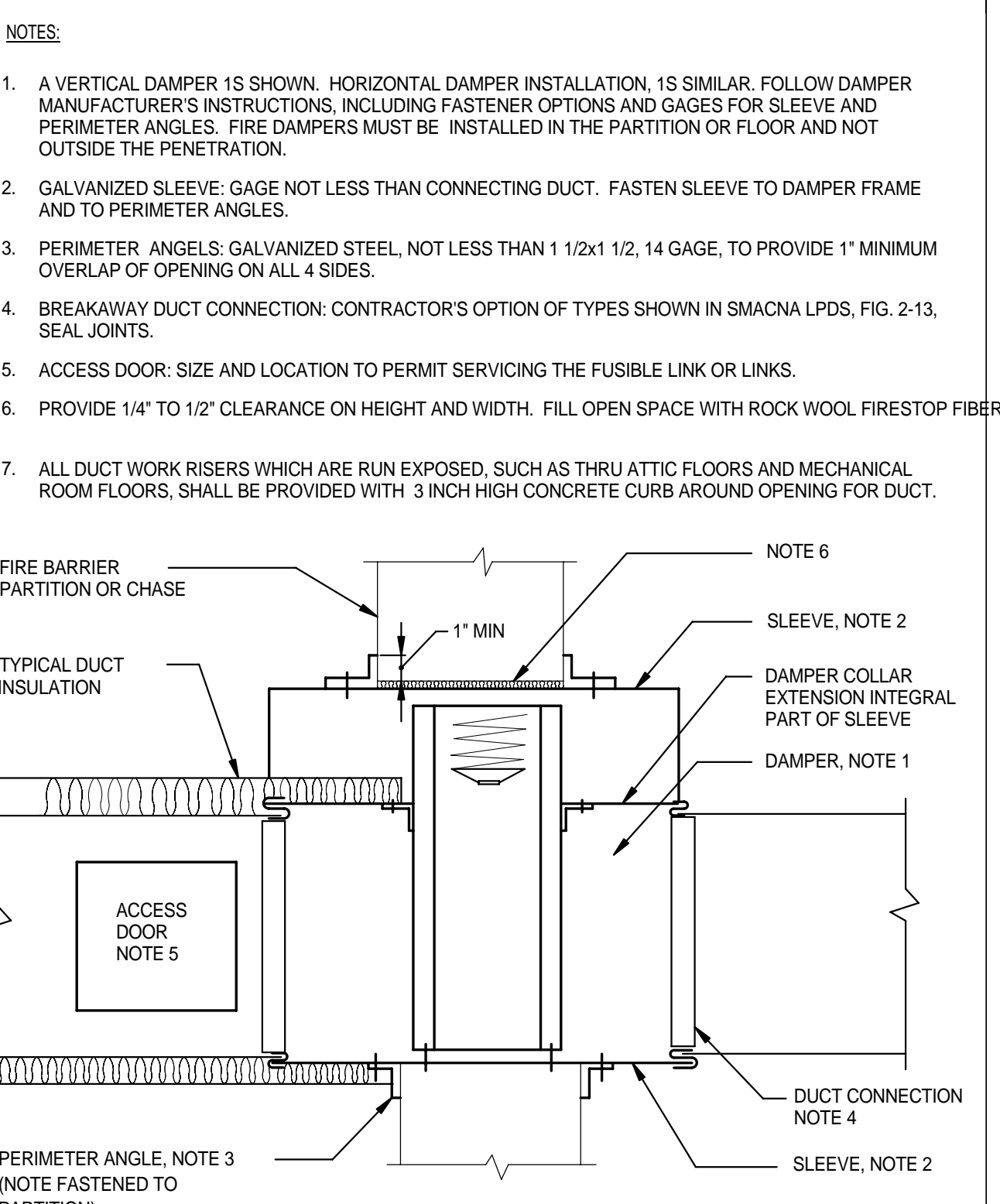
FIRE DAMPER INSTALLATION DETAIL NO SCALE (2) M4-0
