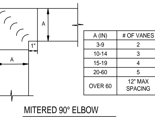
DUCT FITTING DETAILS NO SCALE (11) M4-0
