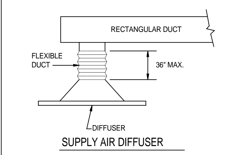
DIFFUSER TAKE-OFF
