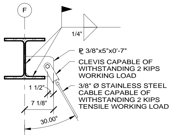
5 CLEVIS PLATE 'B' ELEVATION 1" = 1'-0"
