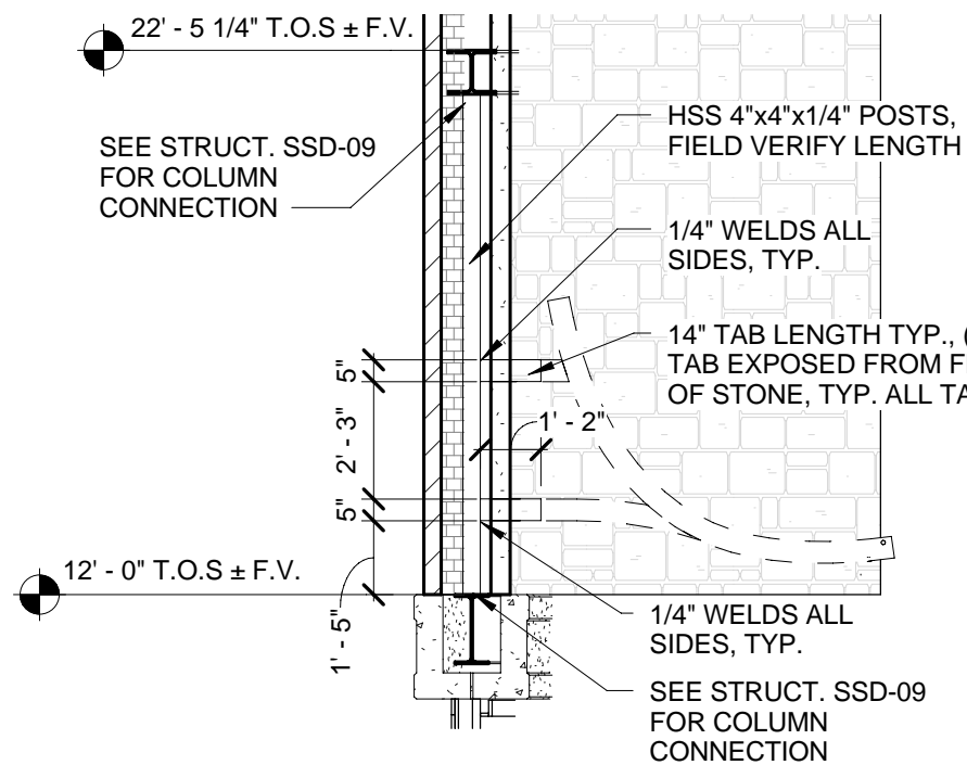
3 Copy of Baptistry Rib - K 1/4" = 1'-0"
