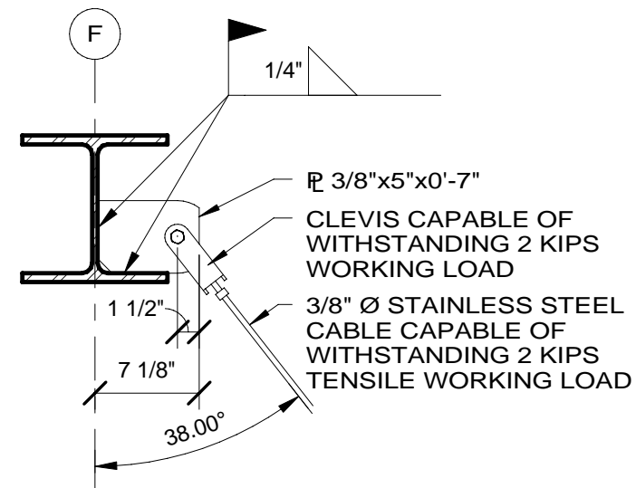
4 CLEVIS PLATE 'A' ELEVATION 1" = 1'-0"
