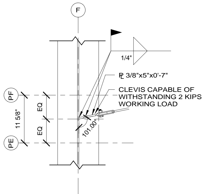
2 CLEVIS PLATE 'B' PLAN DETAIL 1" = 1'-0"
