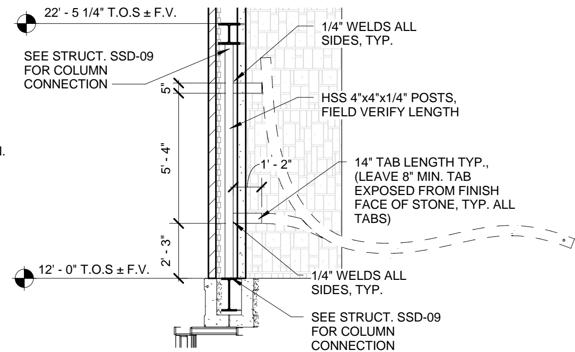
1 Copy of Baptistry Rib - E 1/4" = 1'-0"
