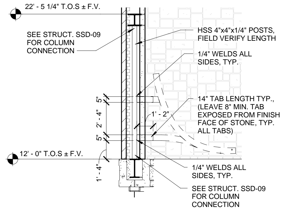
4 Copy of Baptistry Rib - L 1/4" = 1'-0"
