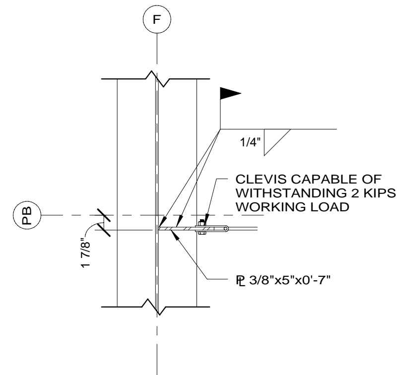
1 CLEVIS PLATE 'A' PLAN DETAIL 1" = 1'-0"
