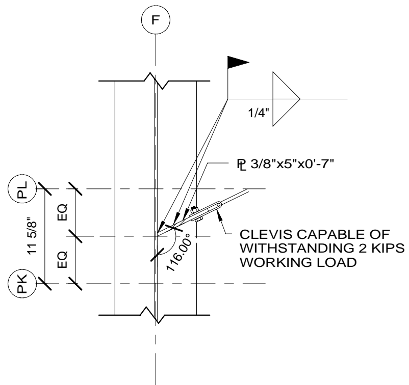
3 CLEVIS PLATE 'C' PLAN DETAIL 1" = 1'-0"
