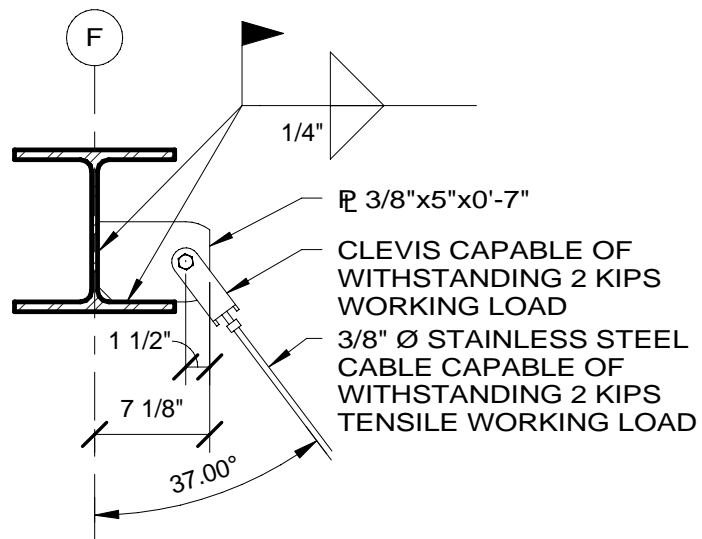
6 CLEVIS PLATE 'C' ELEVATION 1" = 1'-0"
