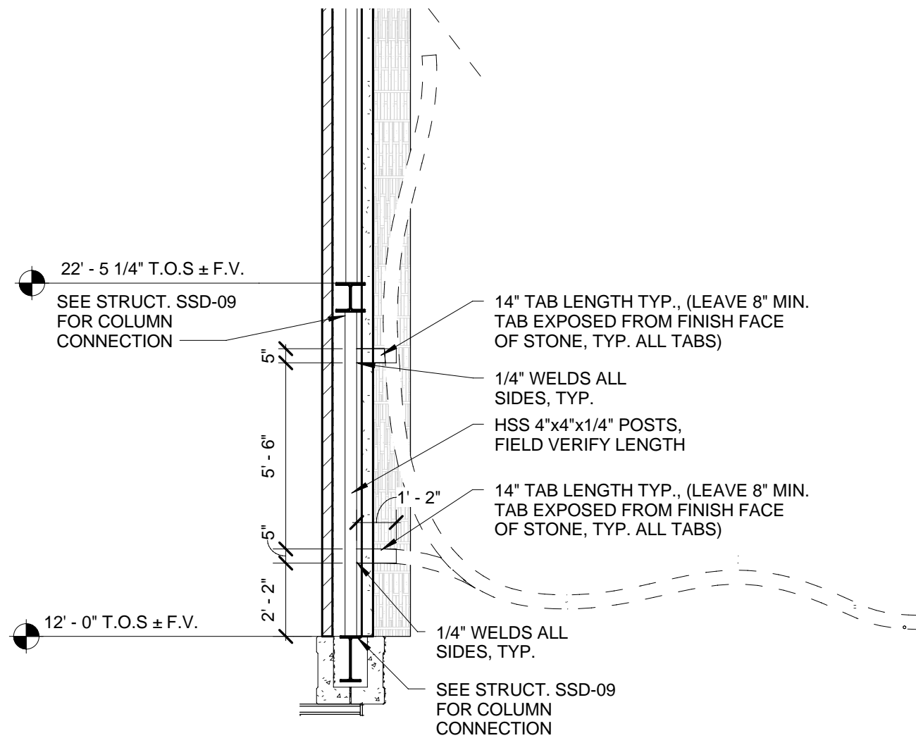
② Copy of Baptistry Rib - B 1/4" = 1'-0"
