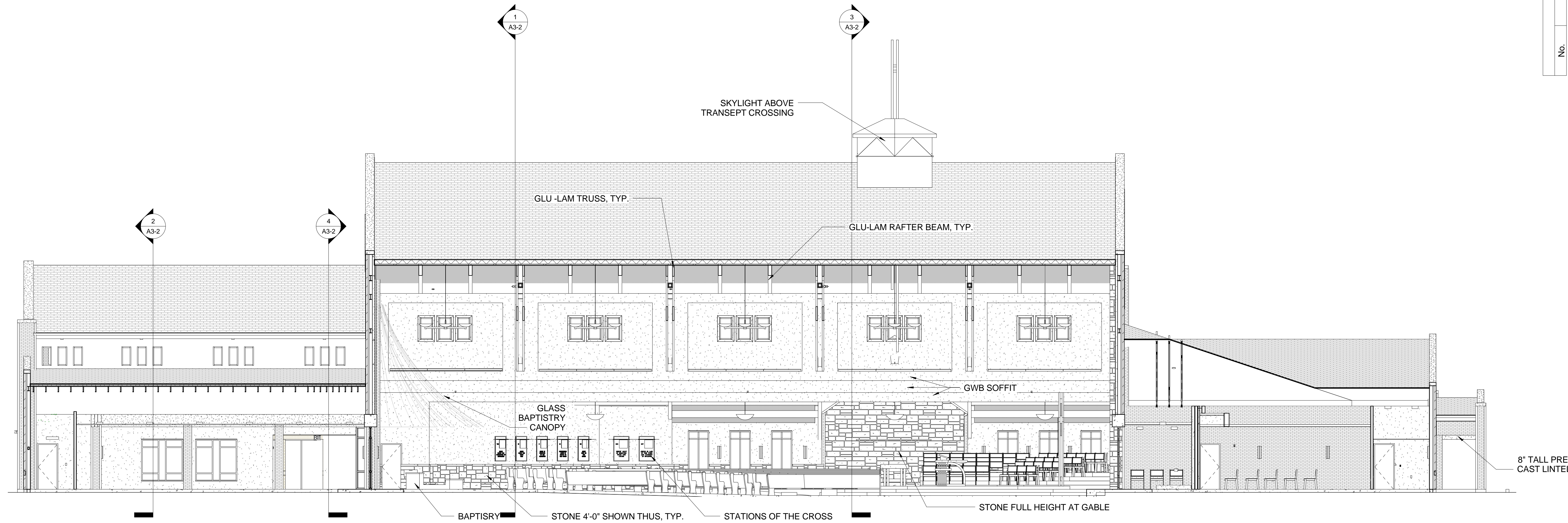
② LONGITUDINAL SECTION, WEST 1/8" = 1'-0"
