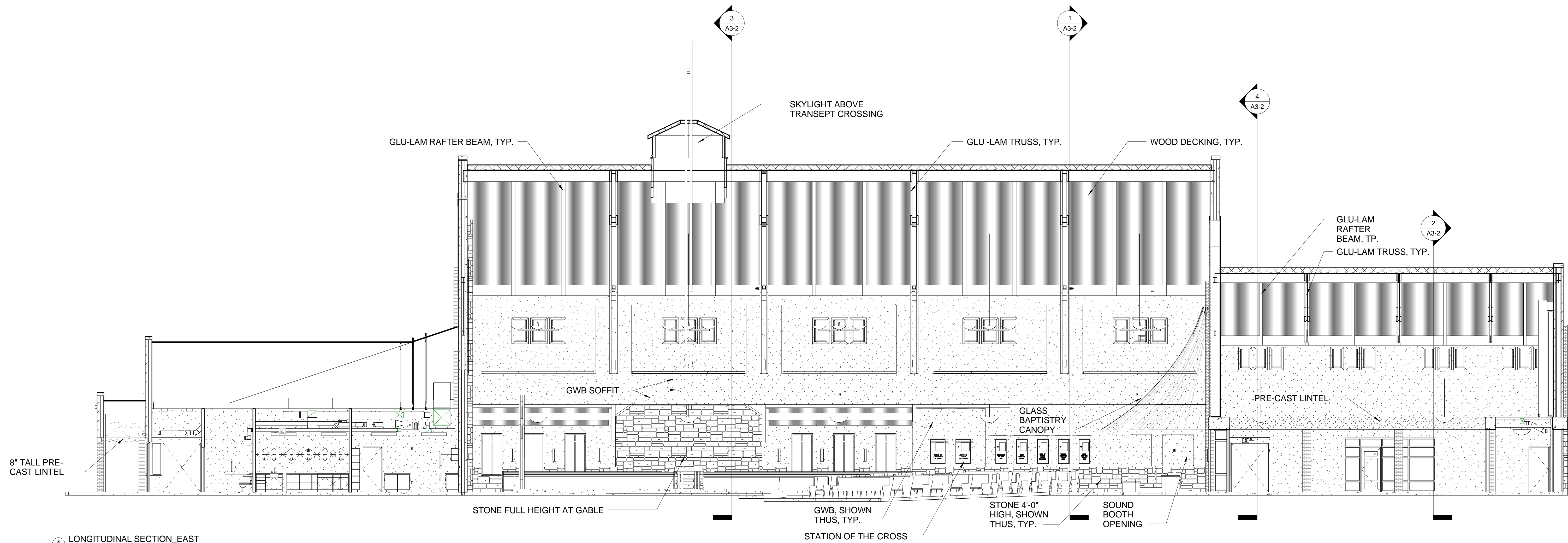
① LONGITUDINAL SECTION, EAST 1/8" = 1'-0"
