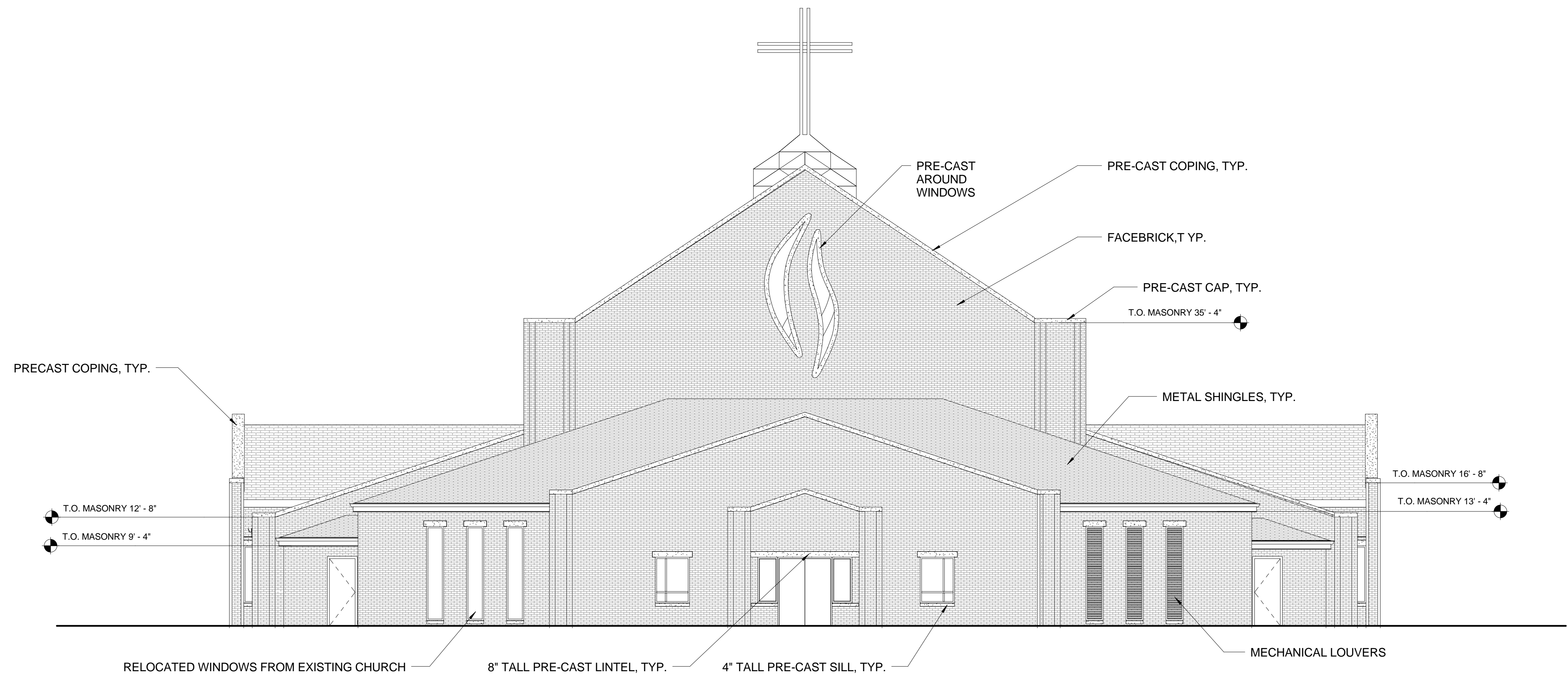
① NORTH ELEVATION 1/8" = 1'-0"
